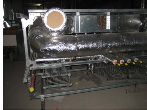
15/5/2009 Ducts: Oxygen, Nitrogen, suction etc IMG_3952.jpg
